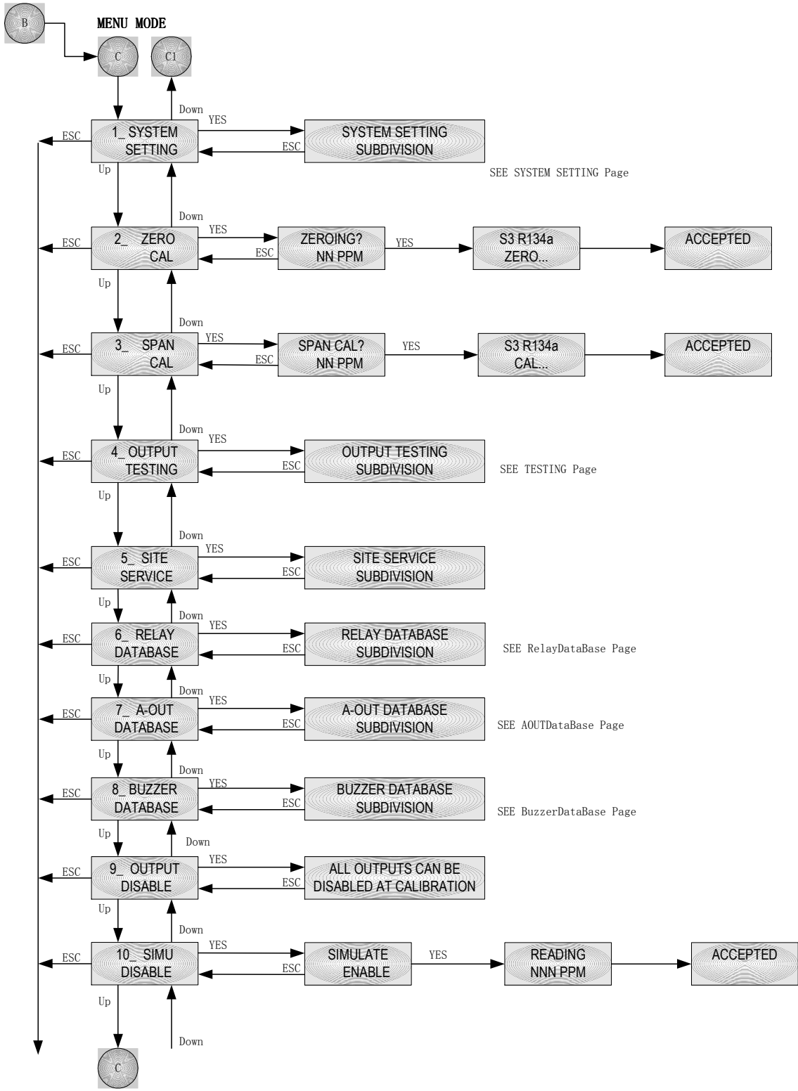
IR-FREON-D Menu Tree Flow Chart
