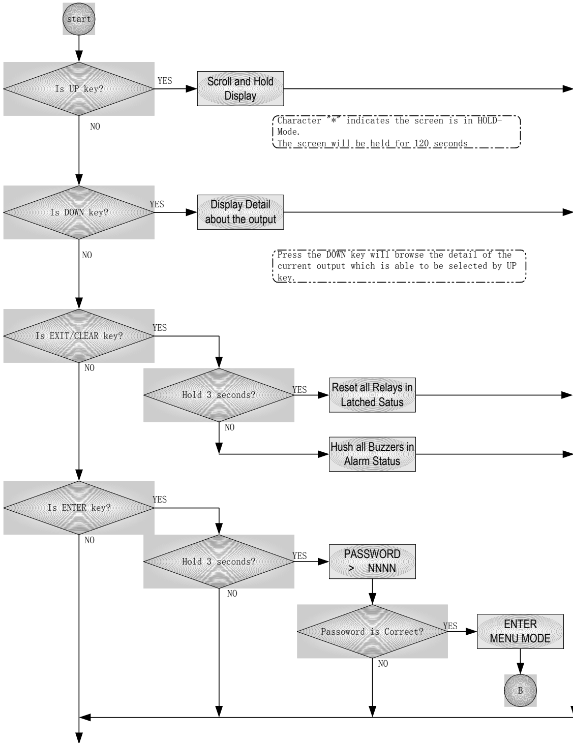
IR-FREON-D Running Mode Key Functions Flow Chart
