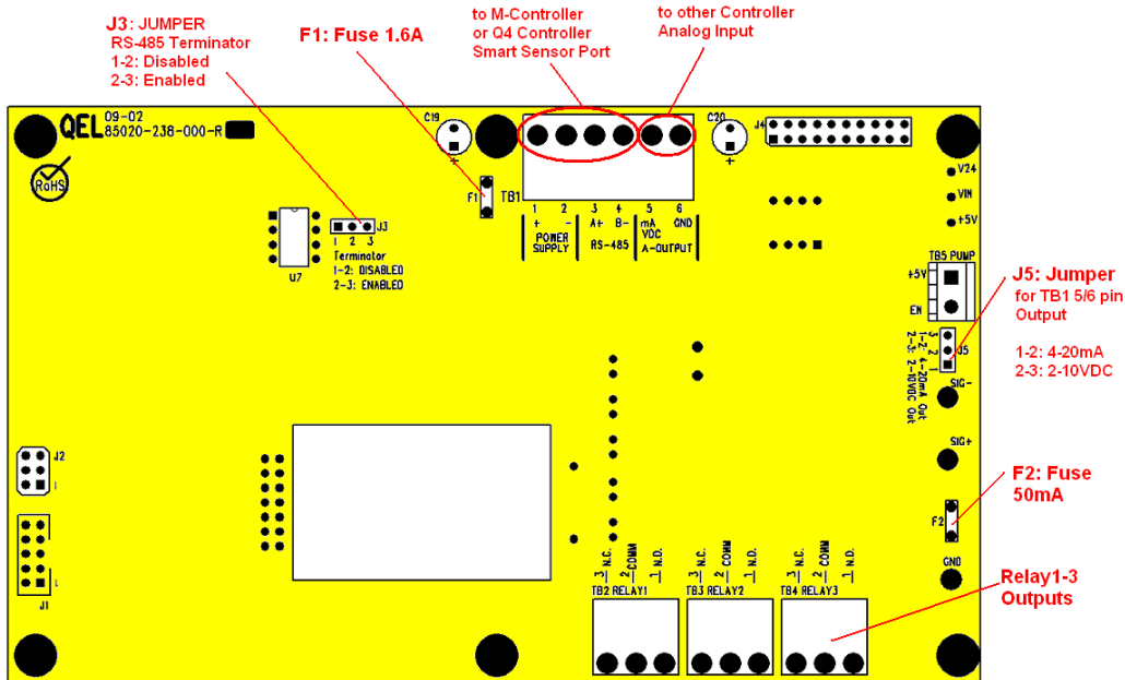
Display Board Terminals
