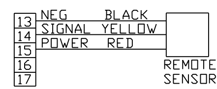
WIRING CONNECTION FOR SOLID STATE SENSOR
