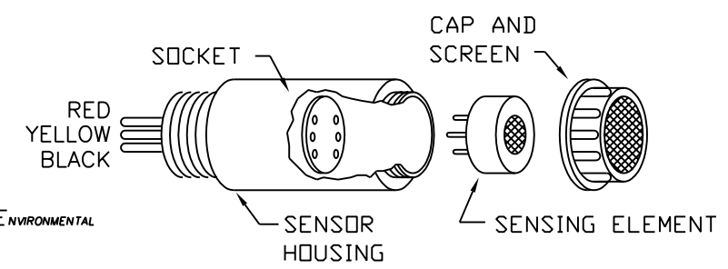
WIRING CONNECTION FOR SOLID STATE SENSOR
